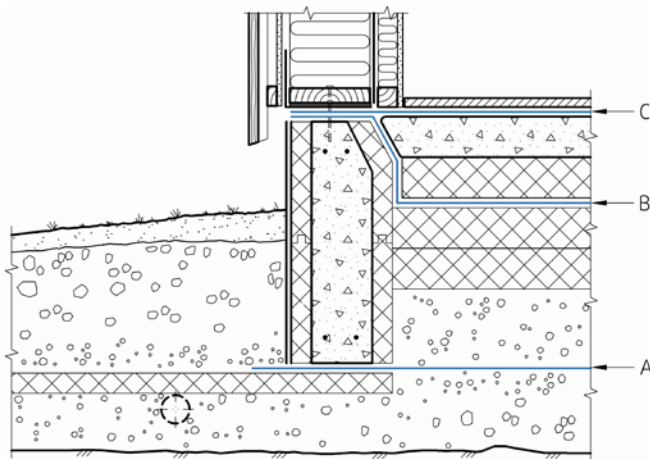
Fig. 1 Example of positioning radon barrier in user group A, B and C.
