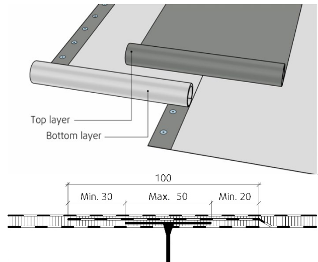
Fig 1 SikaShield® double-layer roof waterproofing membrane. The top layer is fully bonded by welding to the mechanically fixed underlay.
