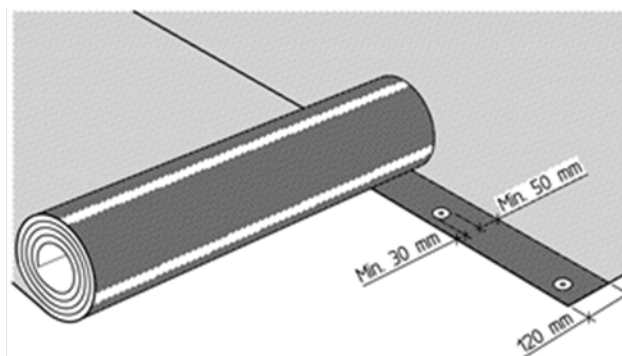
Fig. 1 SikaBit® Pro T-645 mechanically fastened in a 120 mm fully torched or hot air welded overlap joint.
