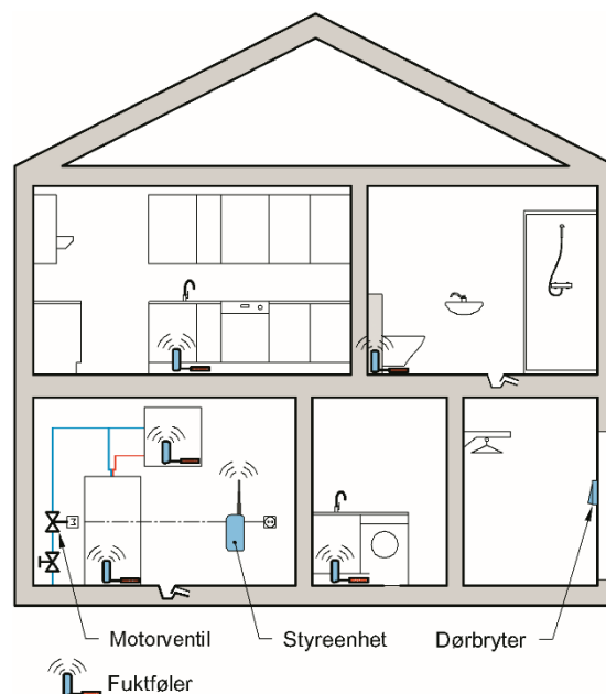
Fig. 1 Systemskisse for WaterStop WS 200 lekkasjestopper
